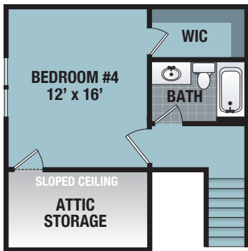
2nd Floor – STANDARD 2384 SQ. FT.
