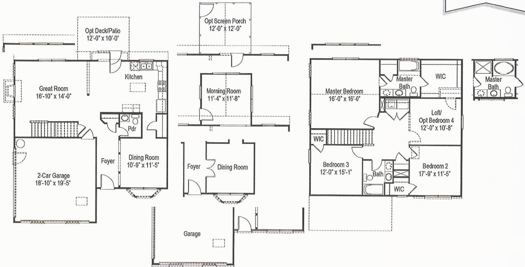
FIRST FLOOR
