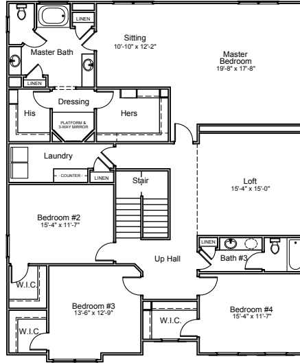
"A" 2nd Floor Plan
