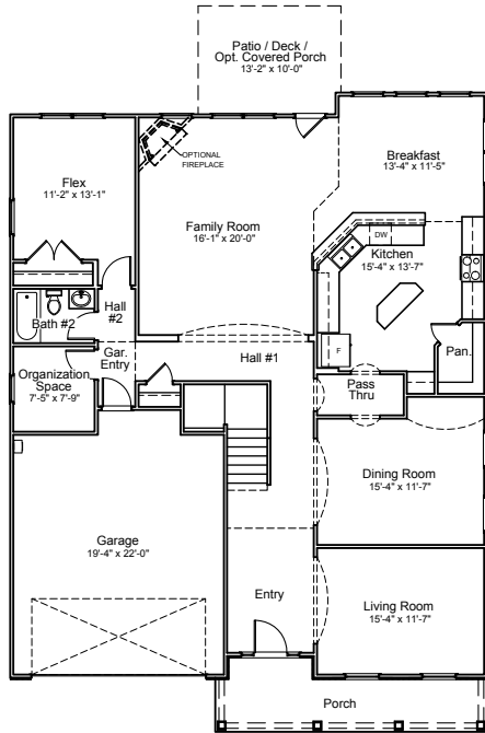
"A" 1st Floor Plan
