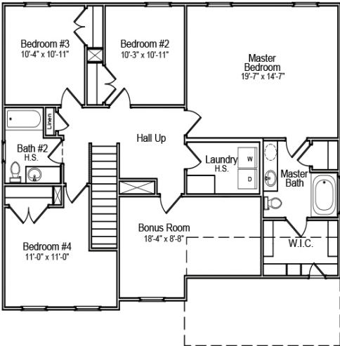
"A" 2nd Floor Plan
