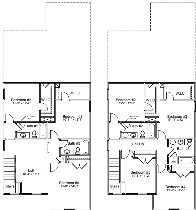
"A" 2nd Floor Plan
