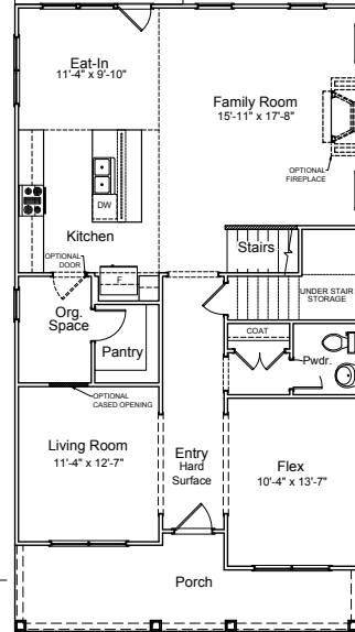
"A" 1st Floor Plan
