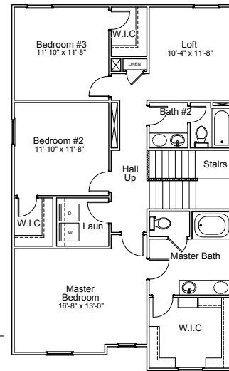
"A" 2nd Floor Plan
