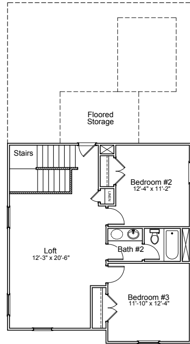
"A" 2nd Floor Plan
