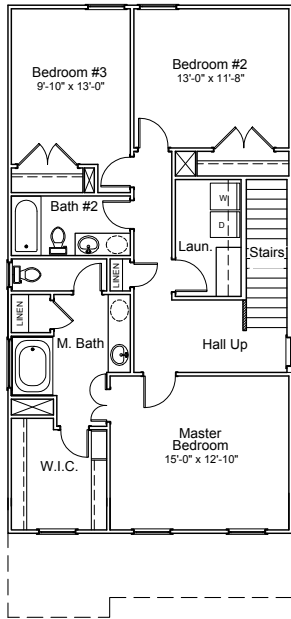
"A" 2nd Floor Plan
