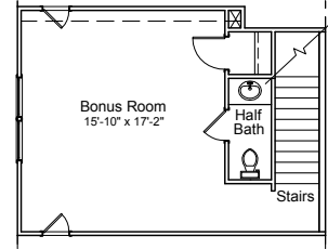
Half Bath Option @ Bonus Room
