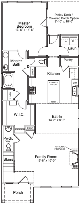
"A" 1st Floor Plan
