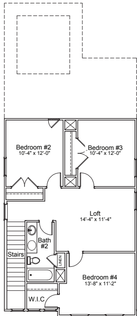
"A" 2nd Floor Plan
