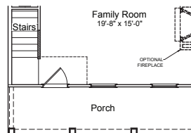
"C" 1st Floor Plan
