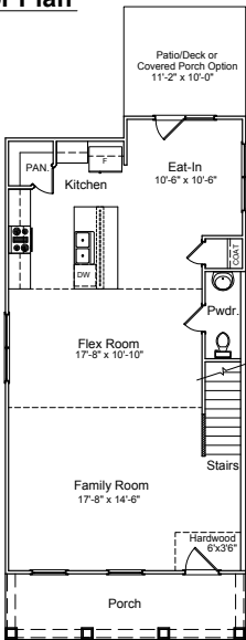
"A" 1st Floor Plan
