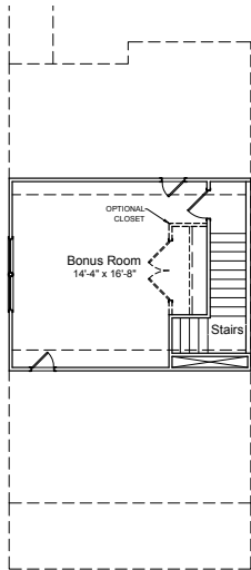
3rd Floor Bonus Room Option
