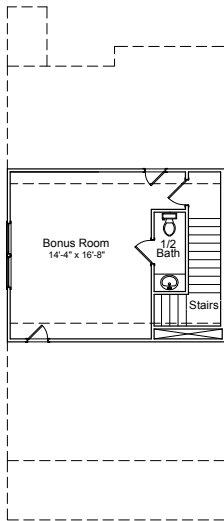
Half Bath Option @ Bonus Room
