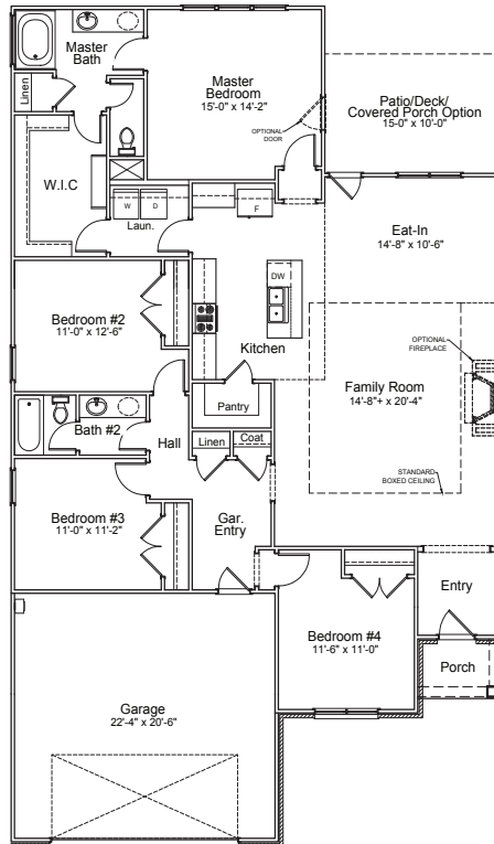
"A" 1st Floor Plan
