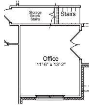
Office Option w/ 2nd Floor Option
